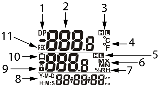
Figure 3.2 Display description.
