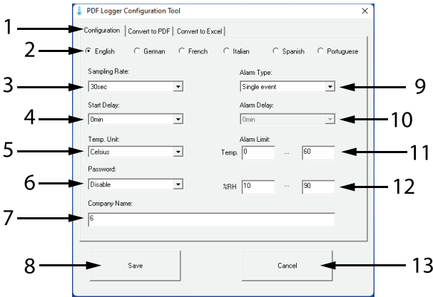
Figure 6.1 PC logger configuration screen. See numbered descriptions in table below.
